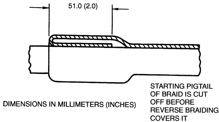
Figure 9-8. Starting Lock
