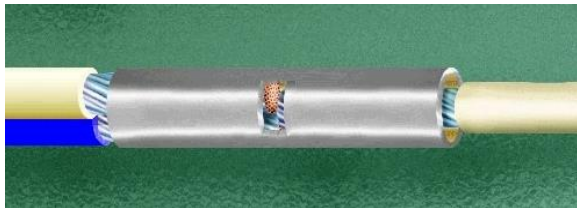
Figure 19-29. Butt Splice Prior to Crimp
